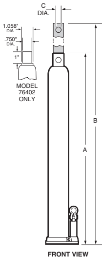
FRONT VIEW
